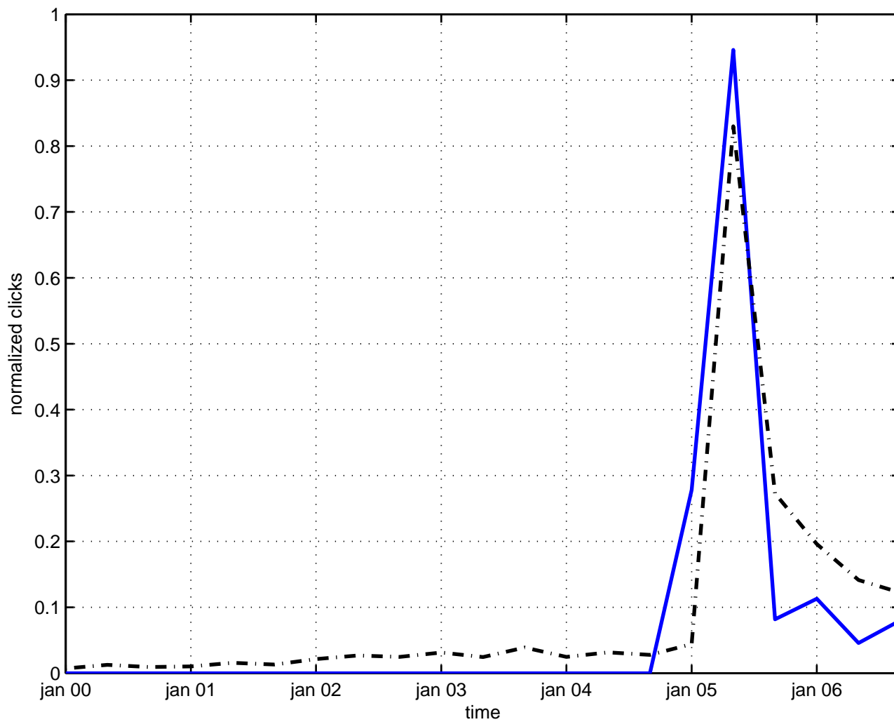
modular localization
