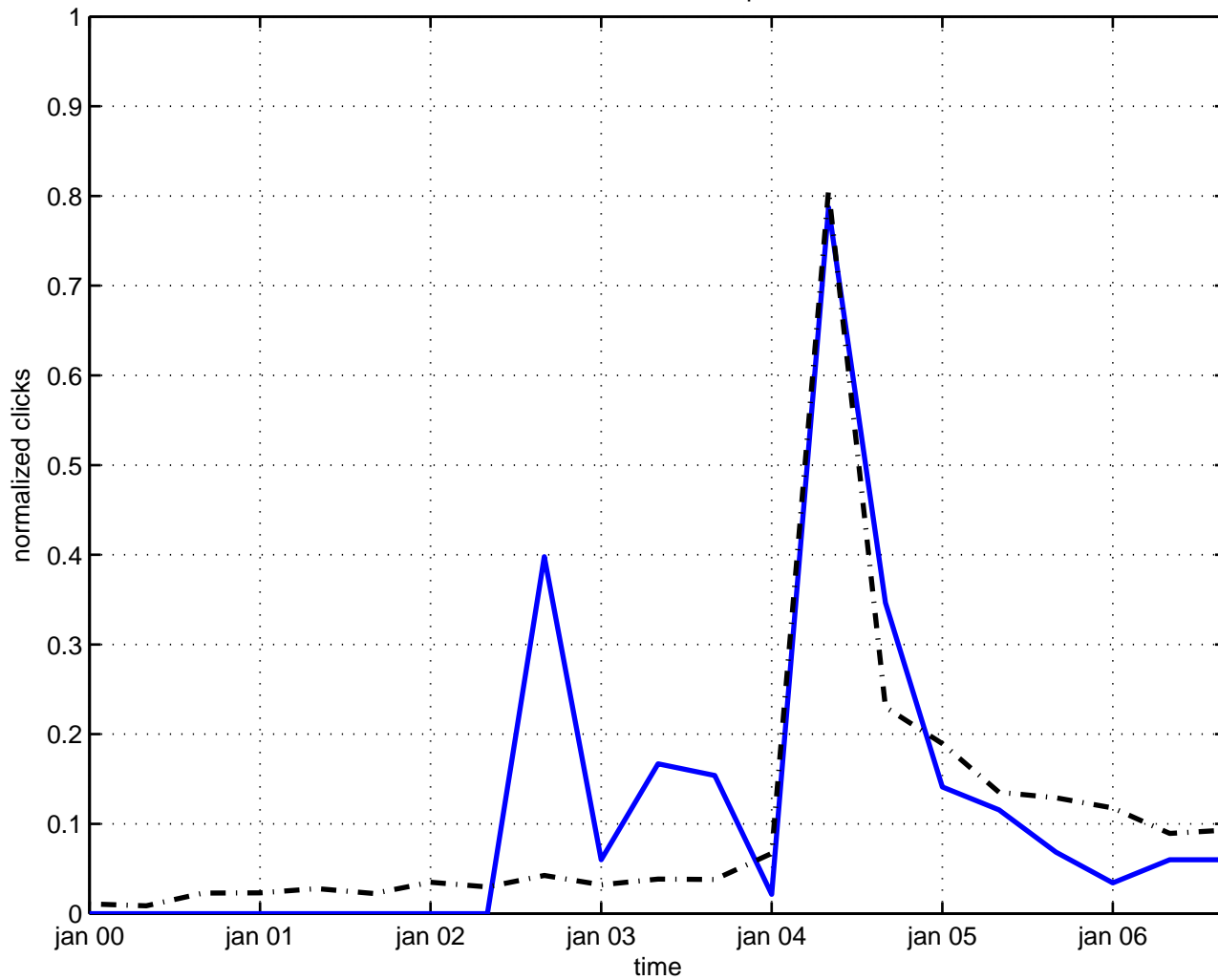
modular bootstrap
