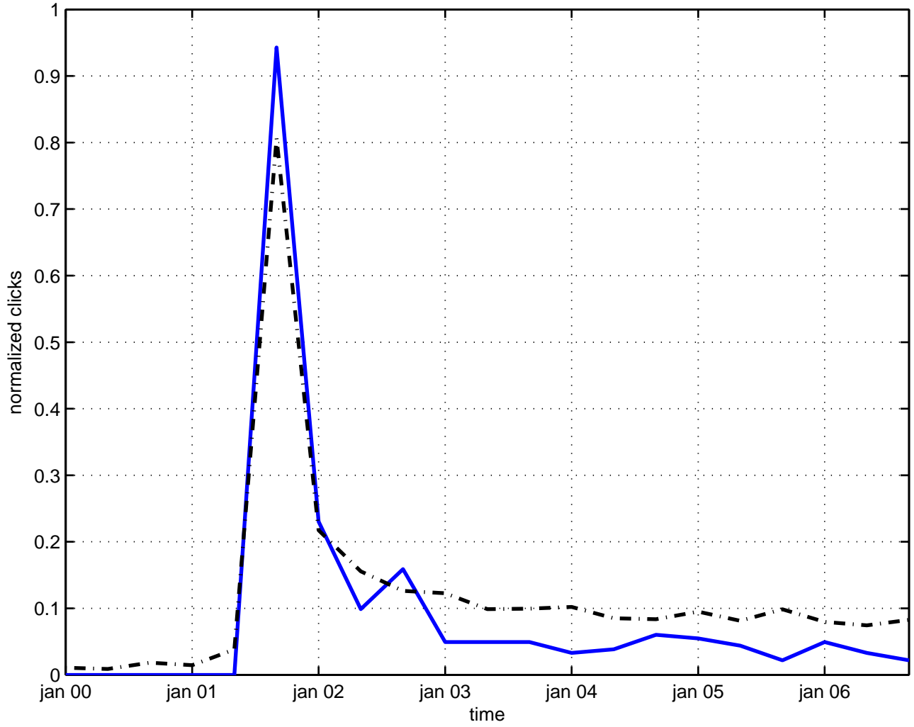
modular anomaly
