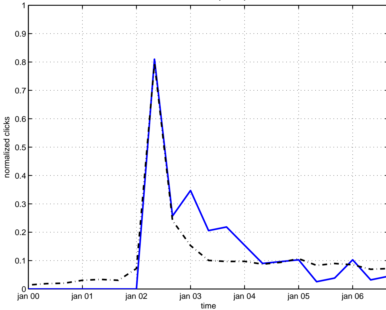
model relativity theory
