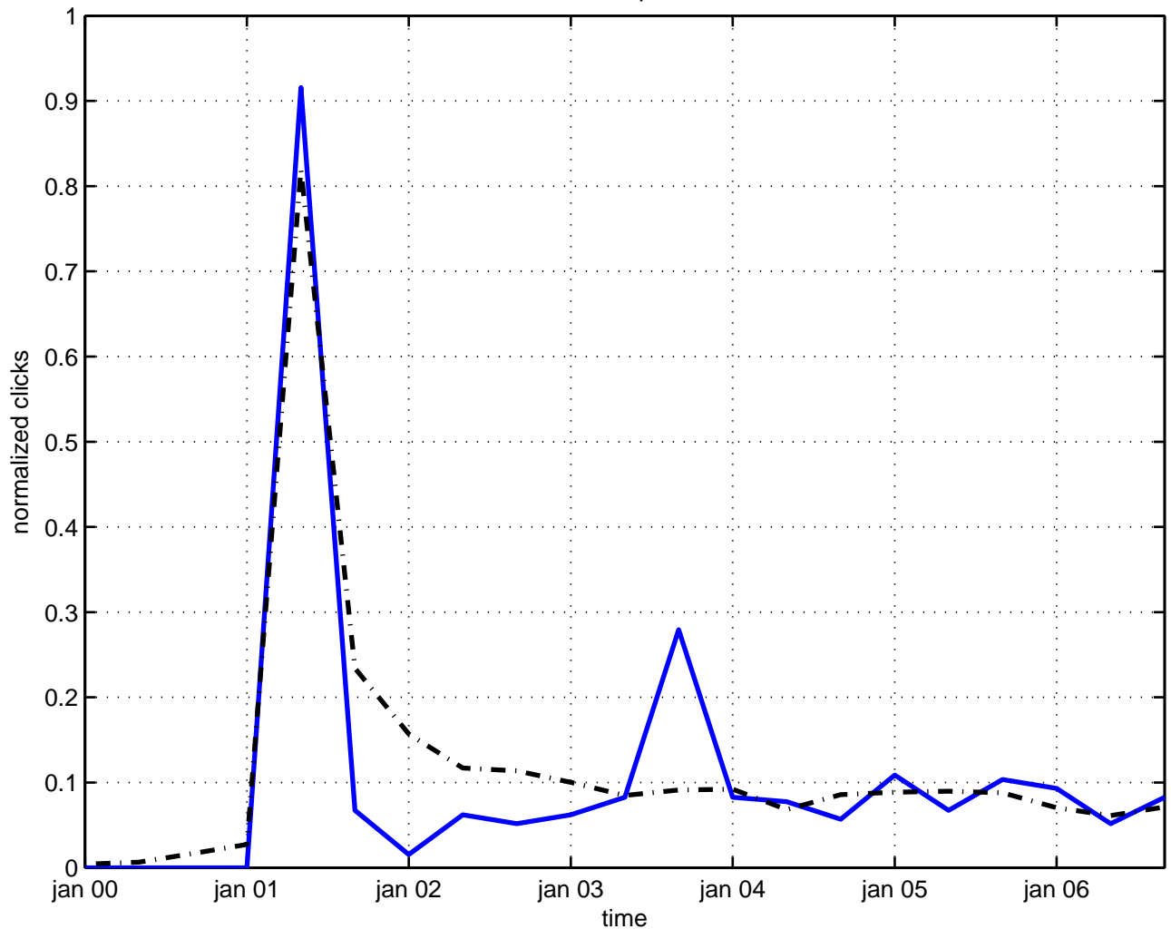
model quark
