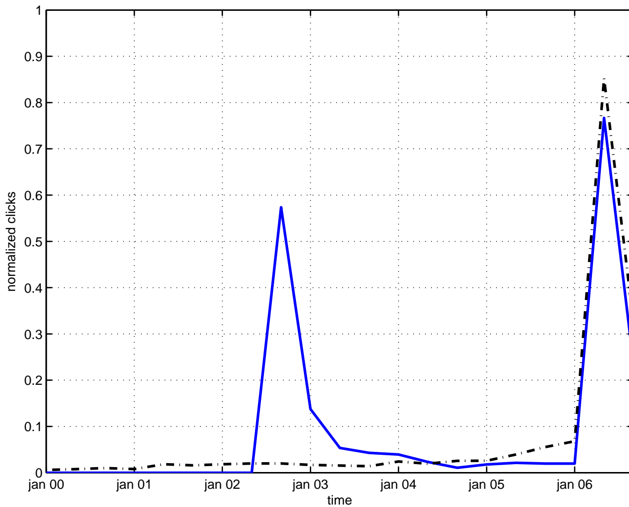
model meson
