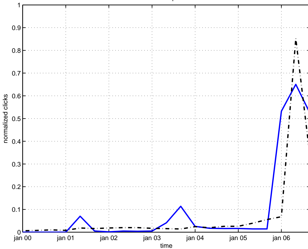
model lepton
