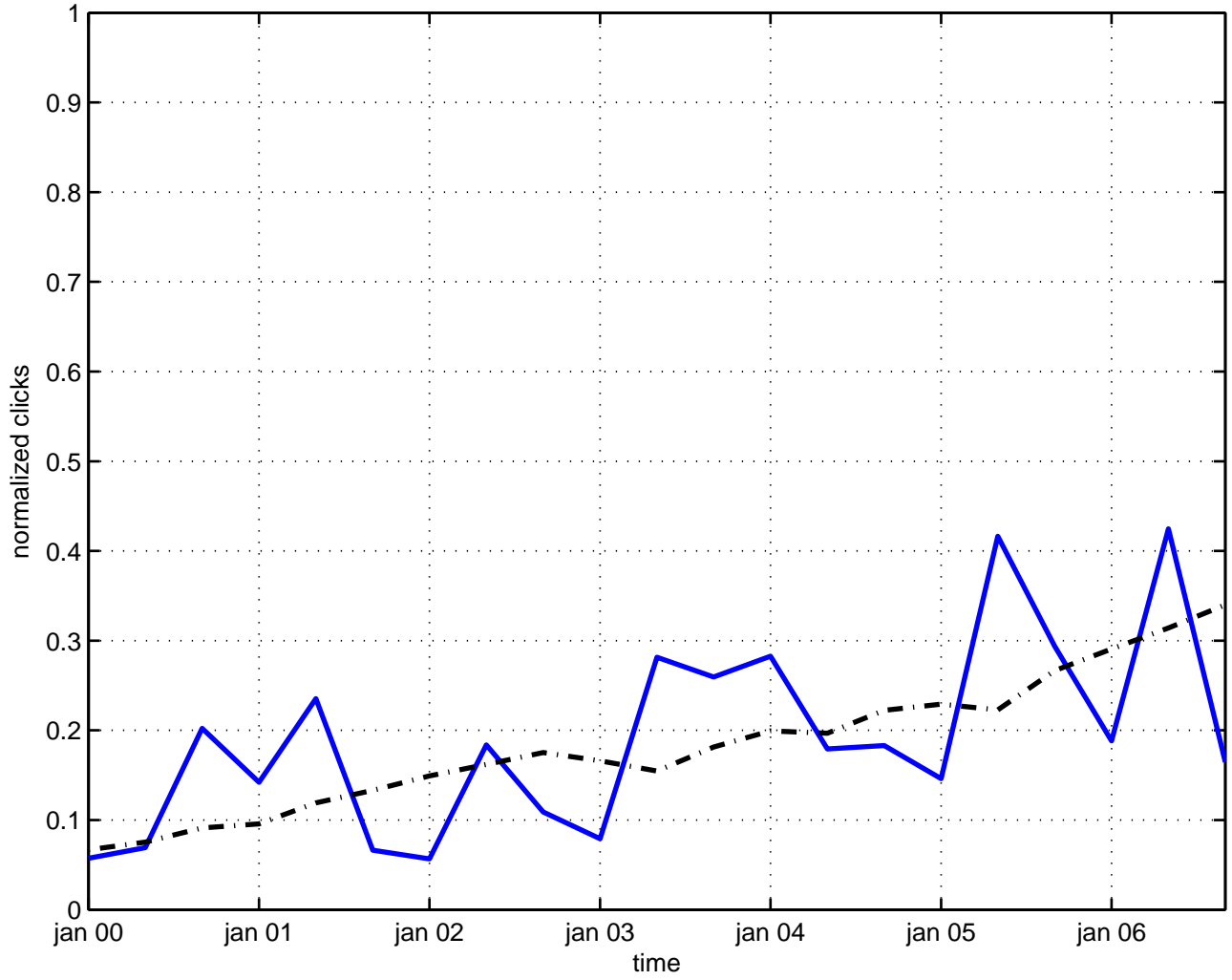
model gravitation
