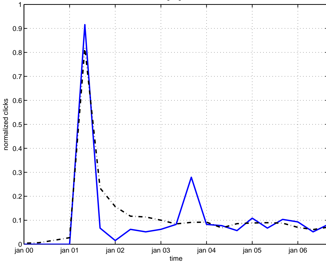
model gauge boson
