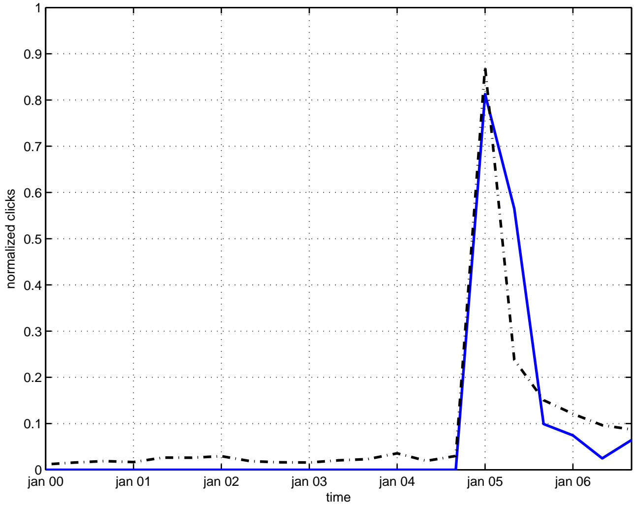
model boson
