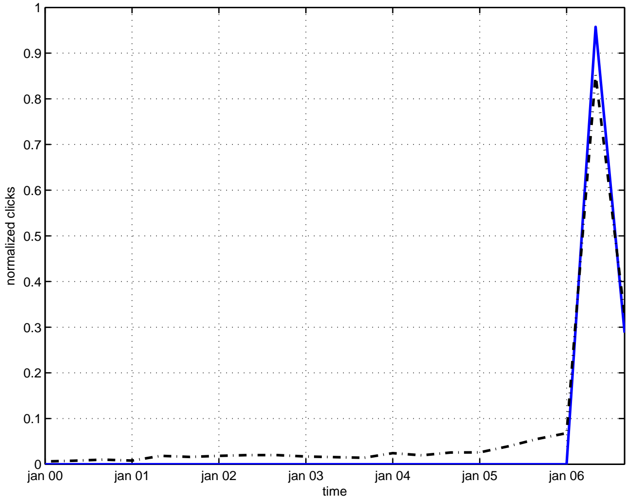
mixing quark
