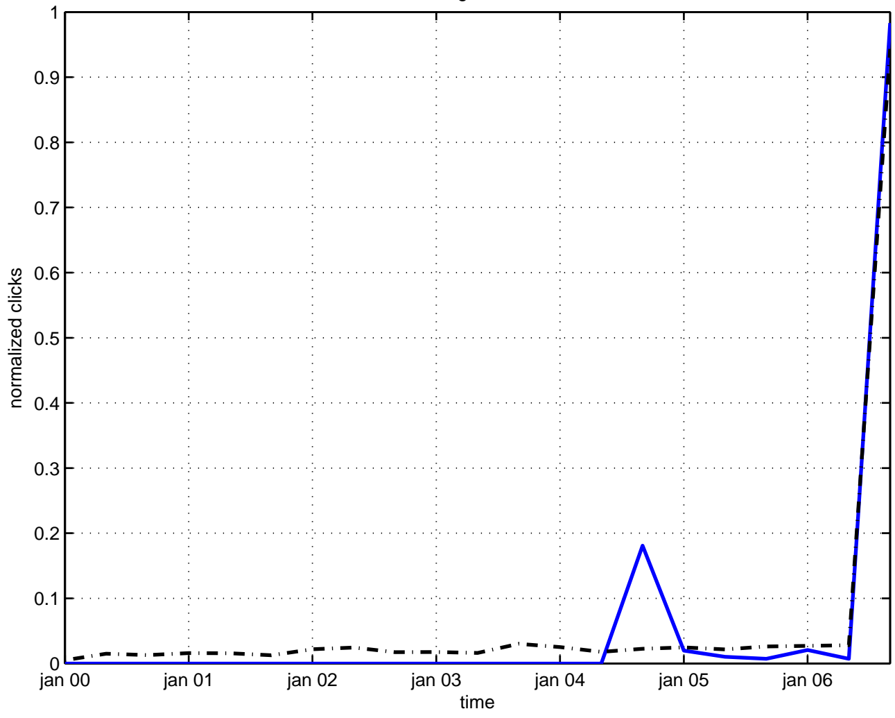
mixing neutrino
