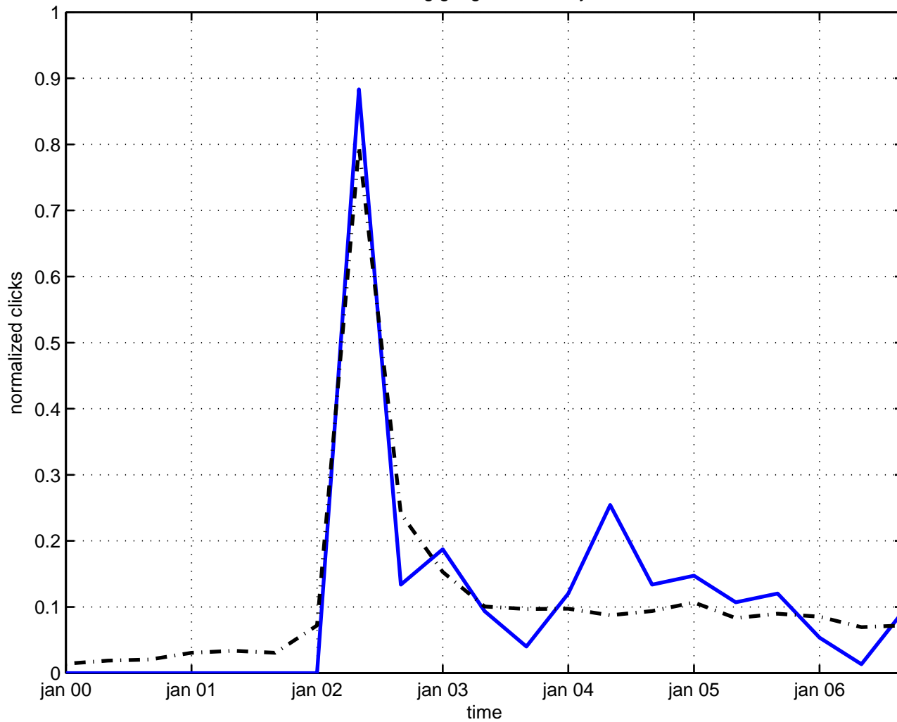
mixing gauge field theory
