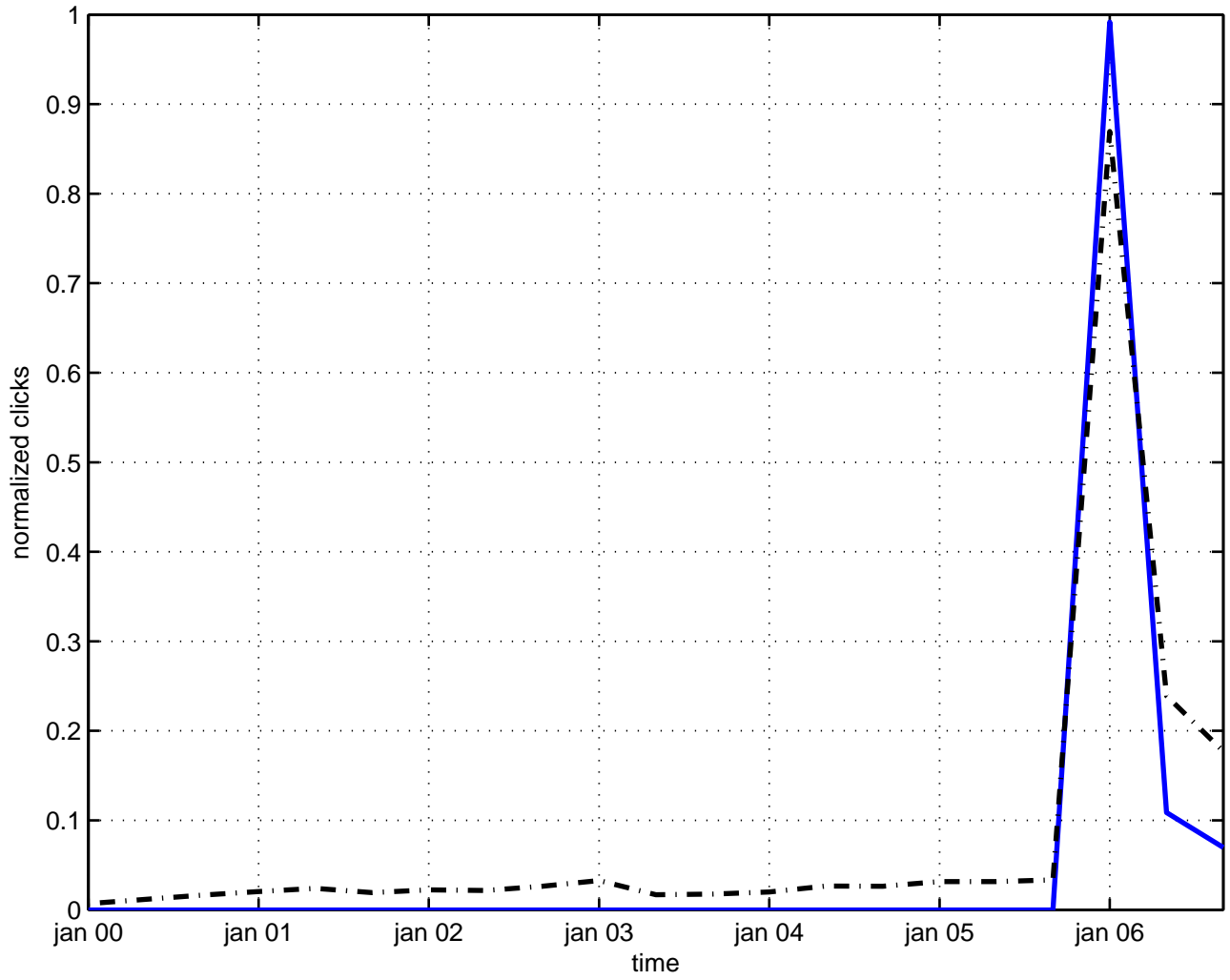
mixing fermion
