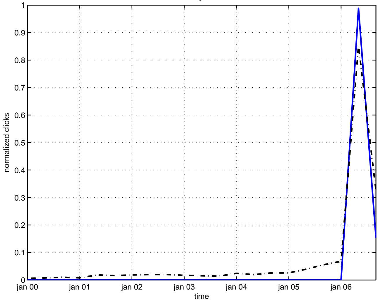
mixing axion
