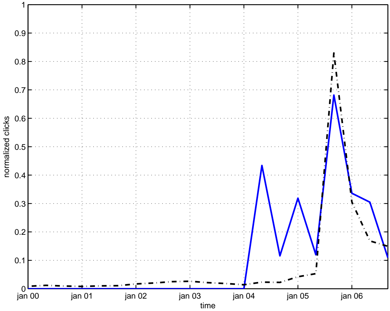
misner space-time
