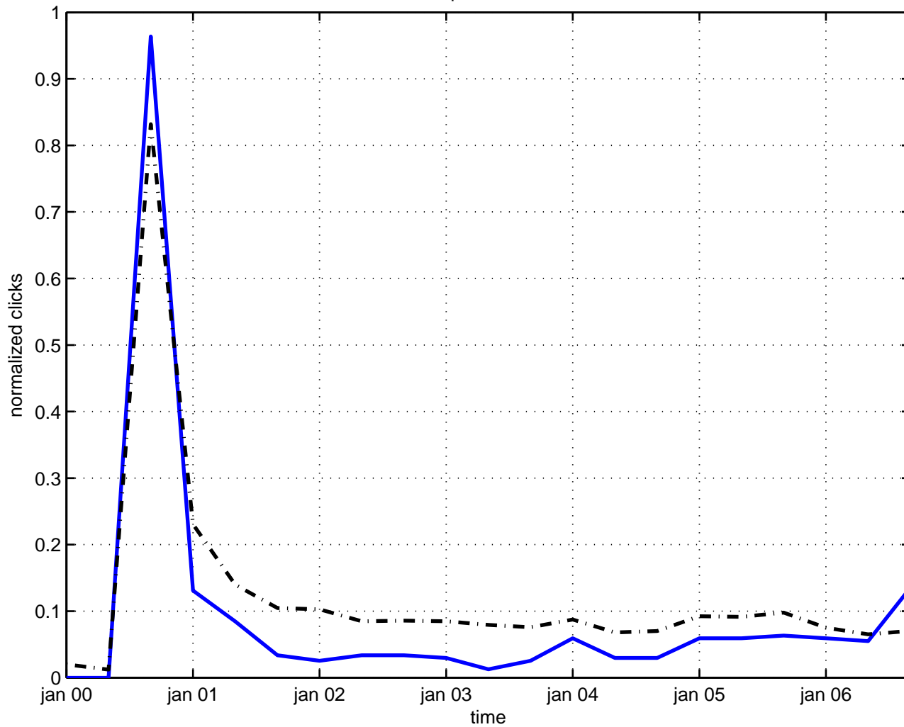
mirror particle fermion
