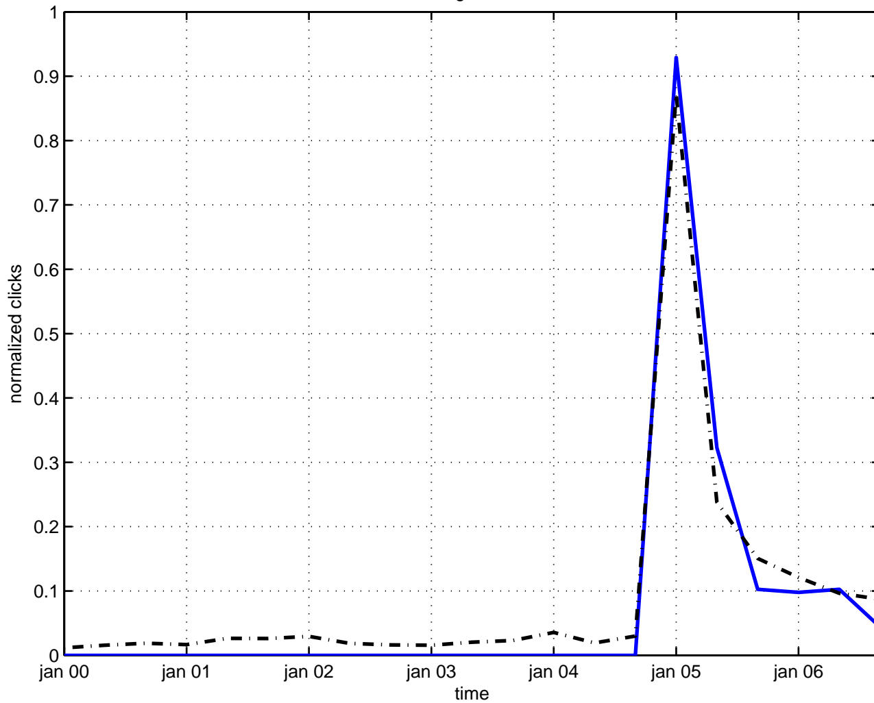
mirage effect
