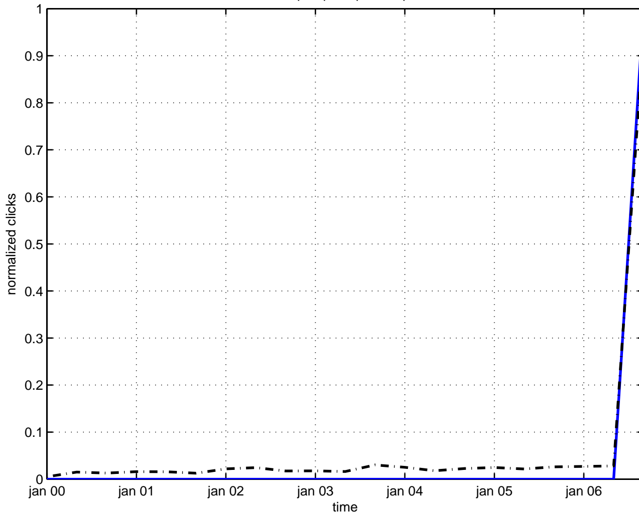
minisuperspace phase space
