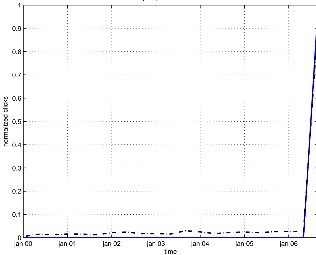
minimal supersymmetric standard model
