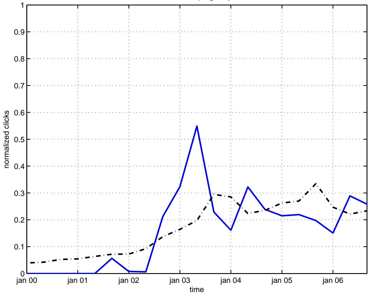
minimal supergravity
