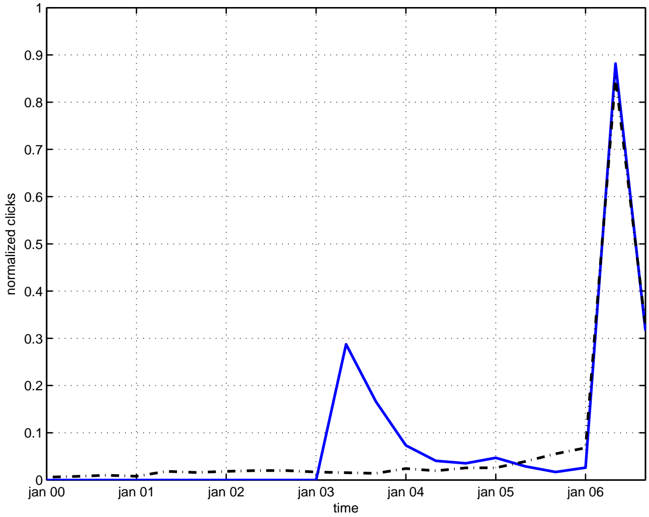
milne orbifold
