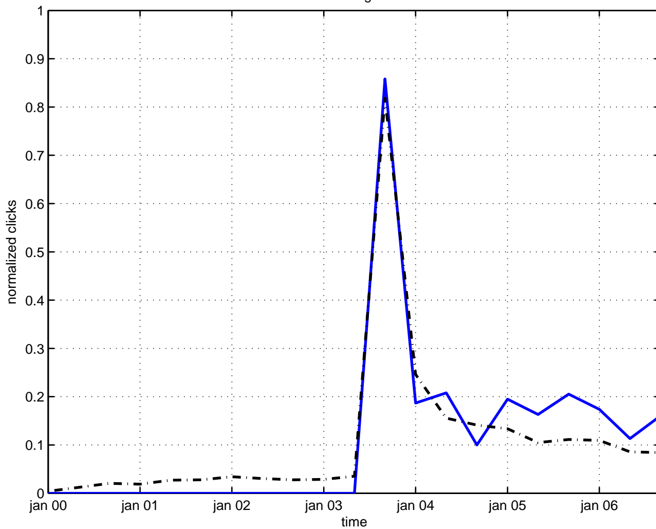
metric-affine gravitation
