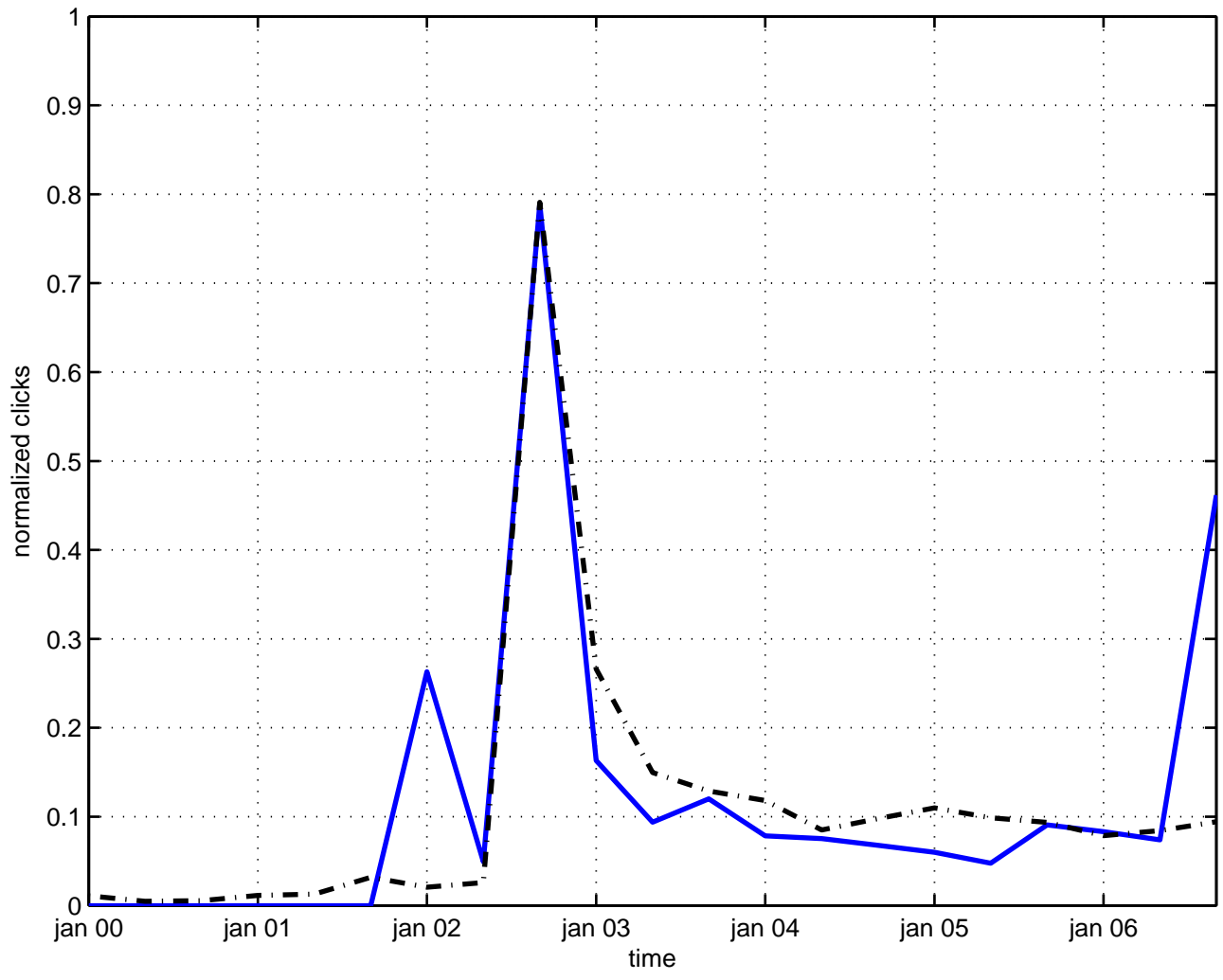
mellin transformation
