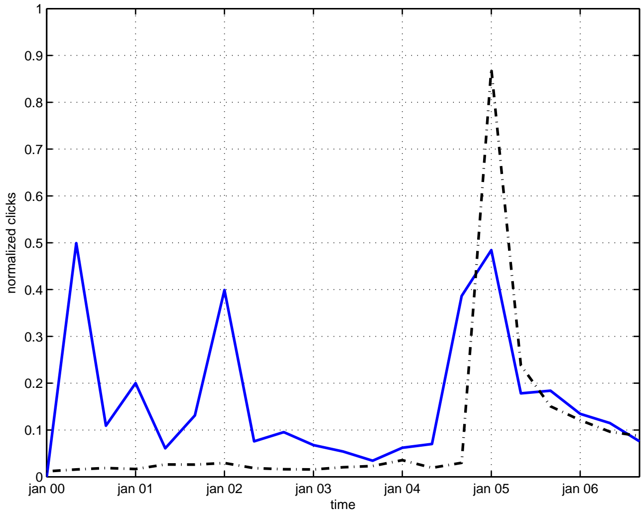
meissner effect
