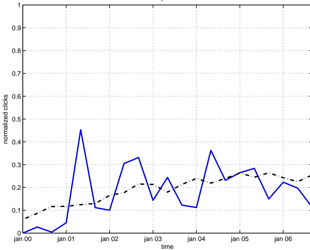
measurement quantum mechanics
