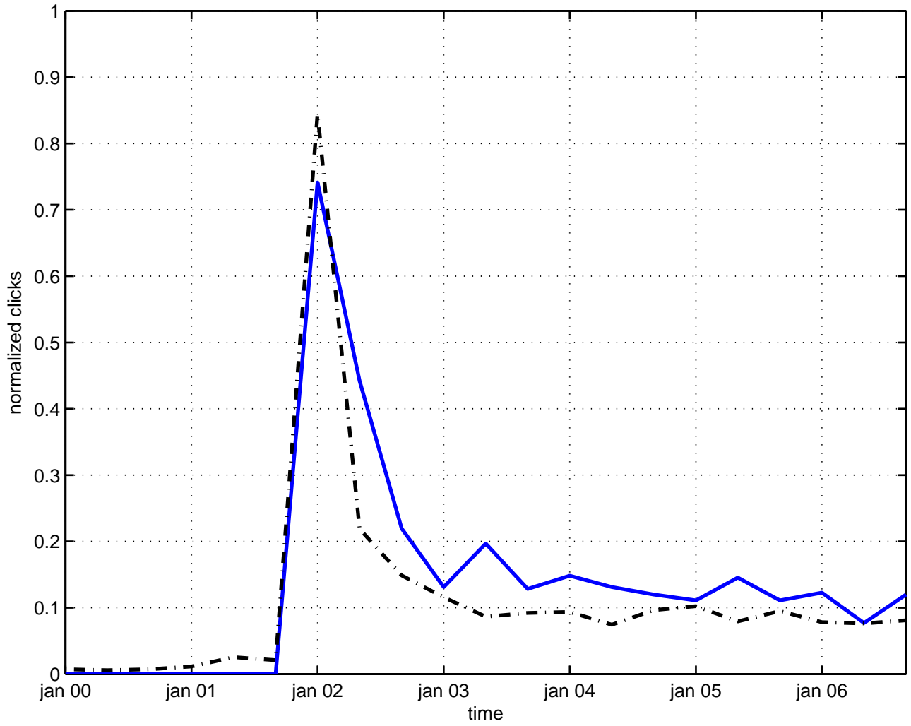
measure instanton
