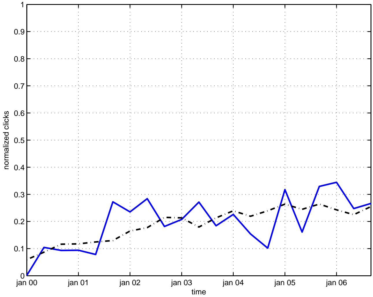
maxwell equation
