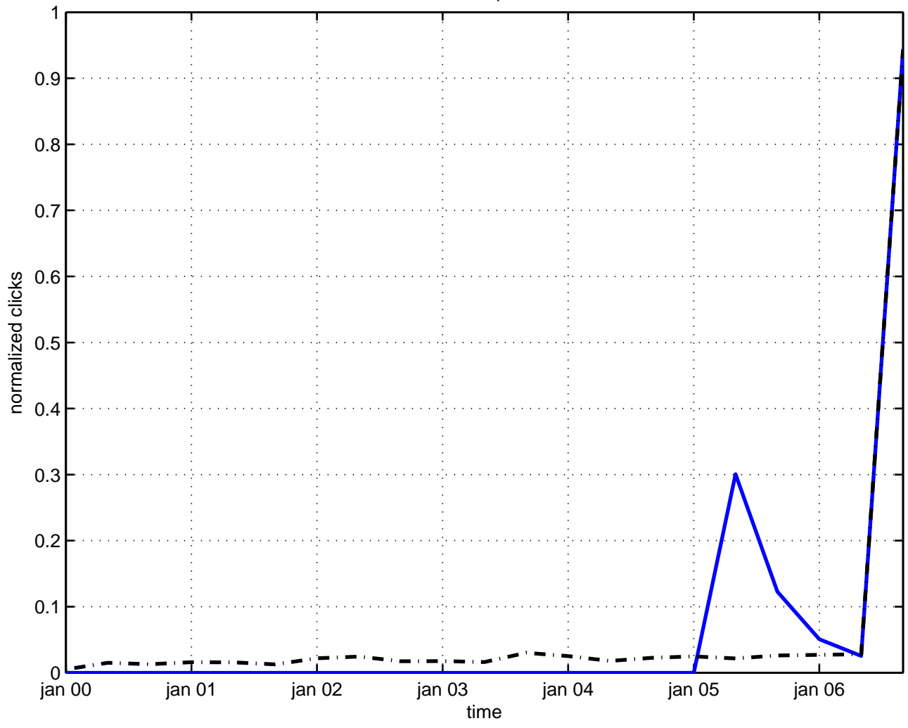
matter quark
