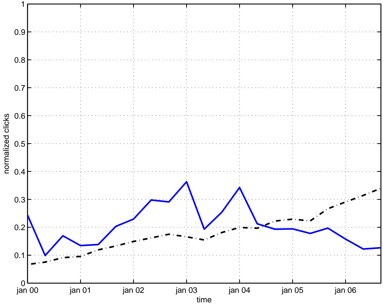
mathematical methods
