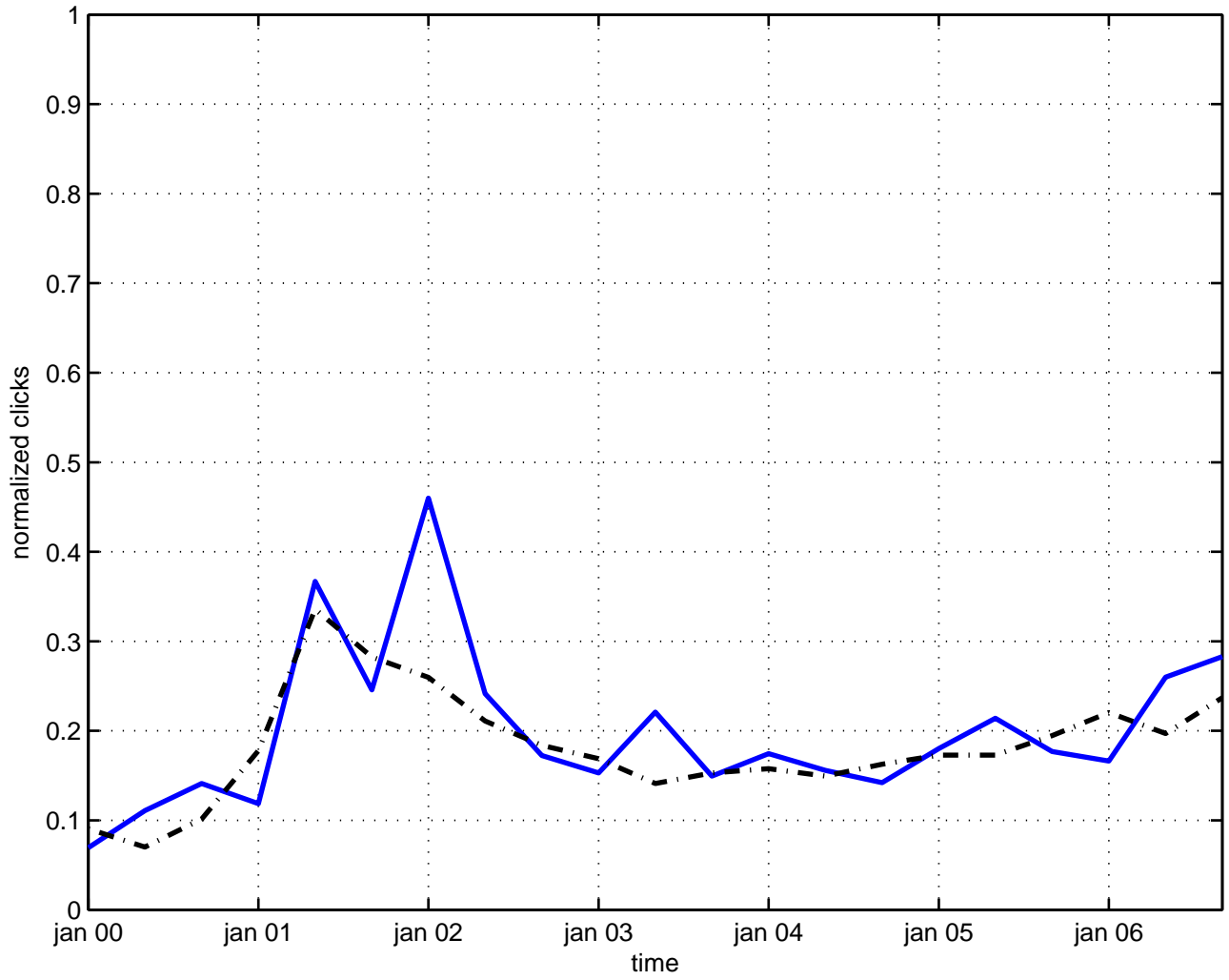
master equation
