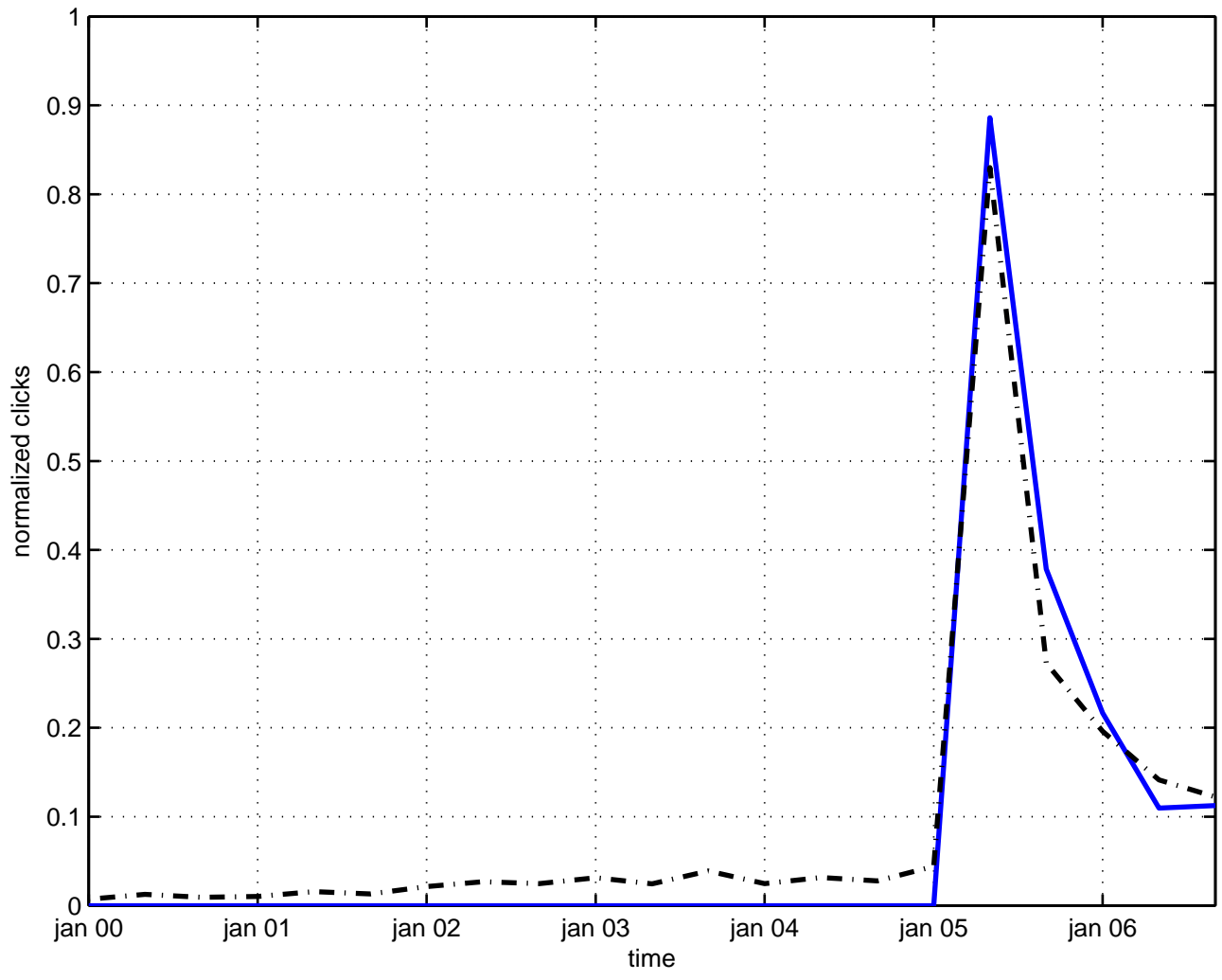
massless zero mode
