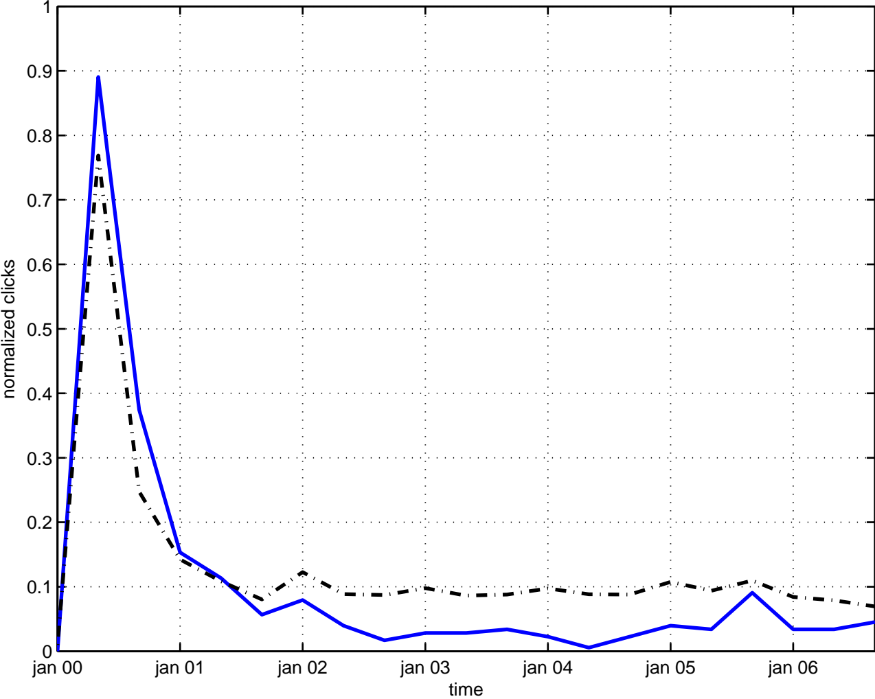
massless wess-zumino model
