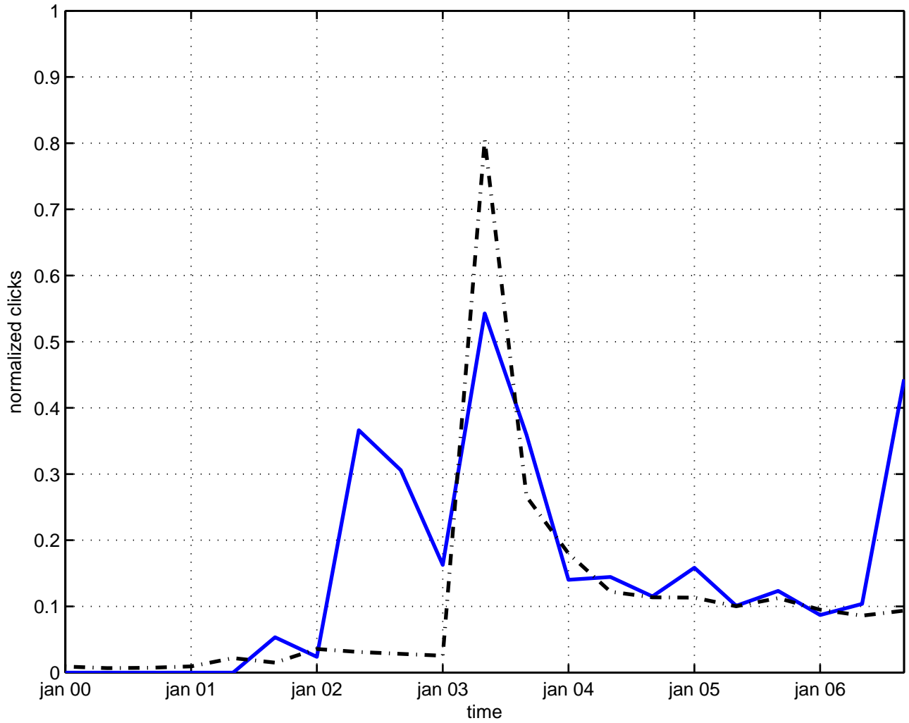
massless thirring model
