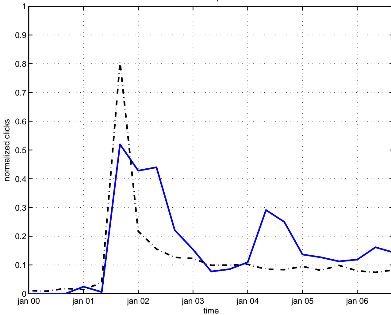
massless spectrum
