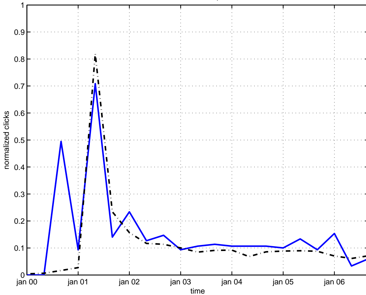
massless multiplet
