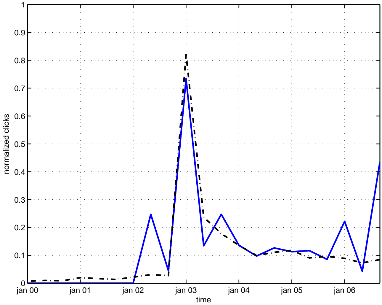
massless boson
