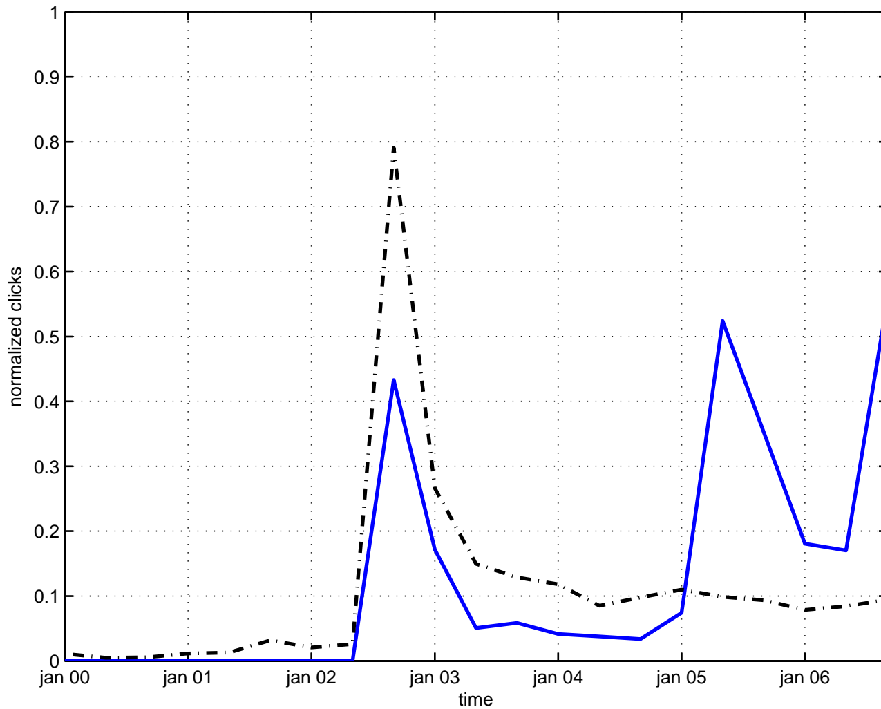
massless black hole
