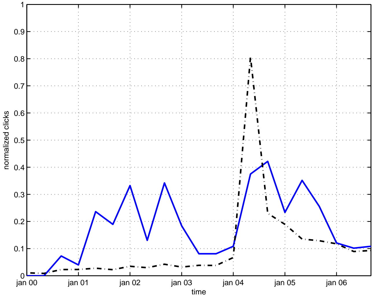
massive supergravity
