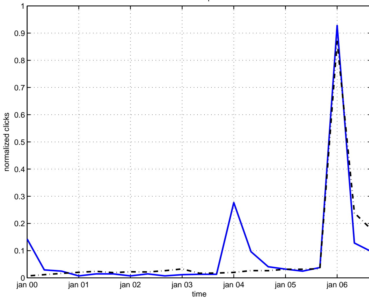
massive spinor
