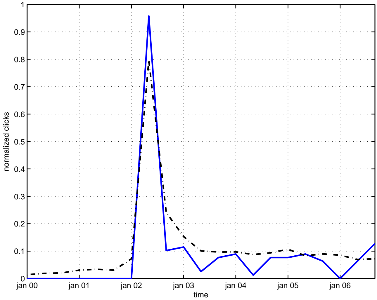
massive quark
