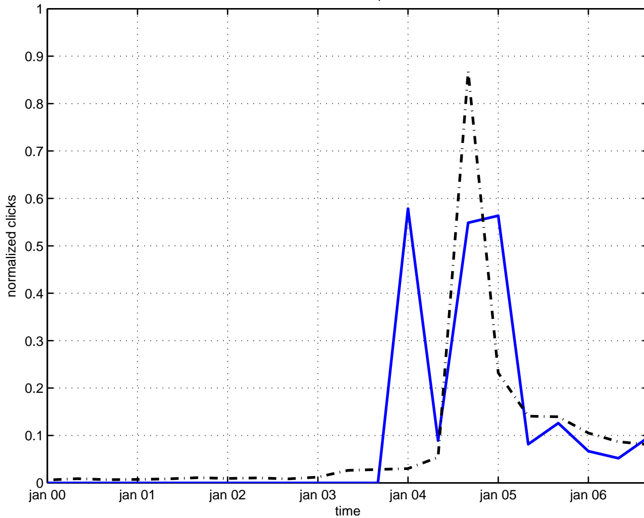
massive multiplet
