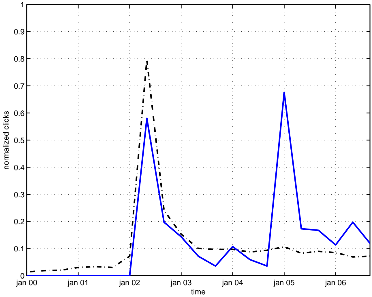
massive magnetic monopole
