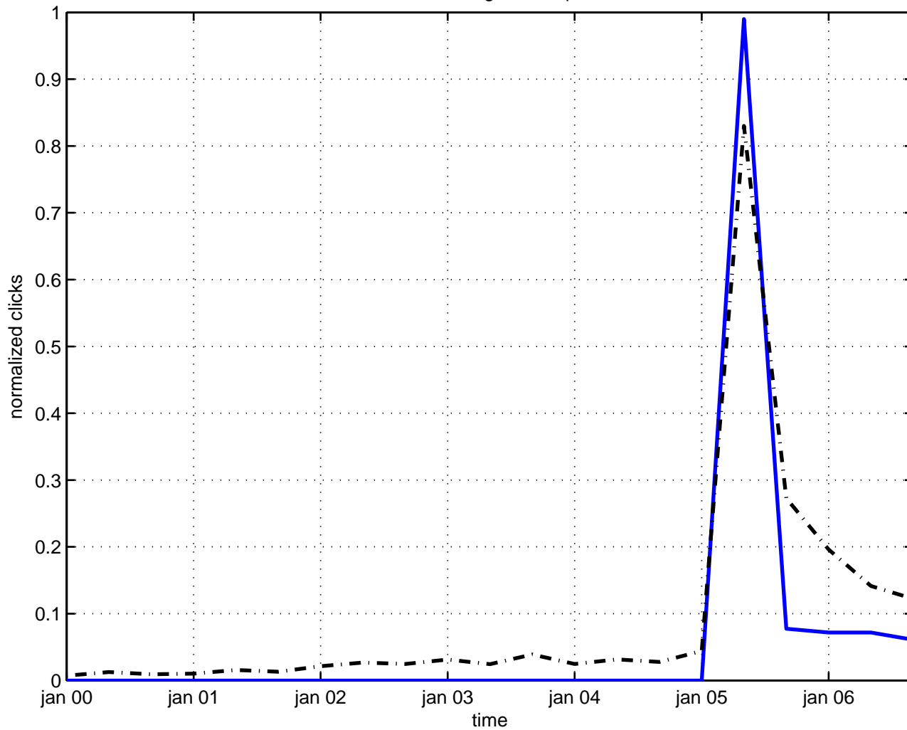
massive klein-gordon equation
