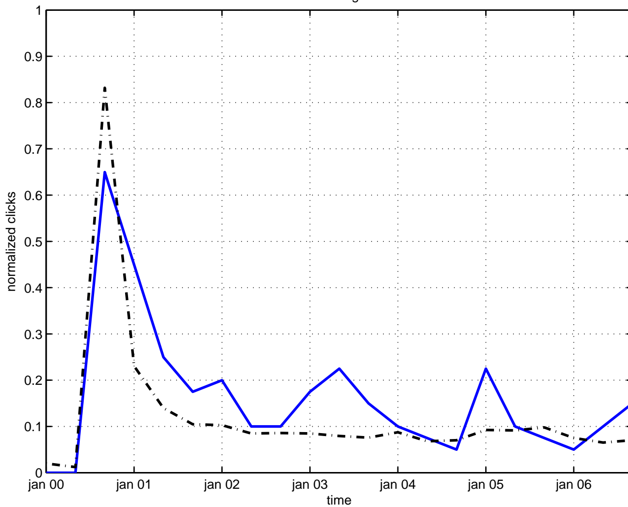
massive ising model
