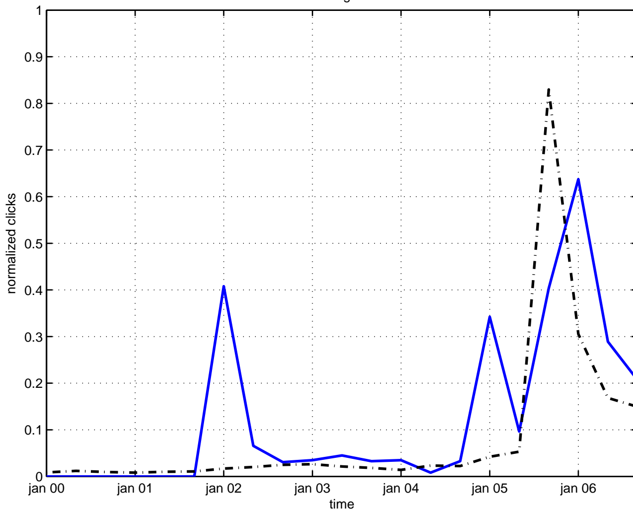
massive gravitino
