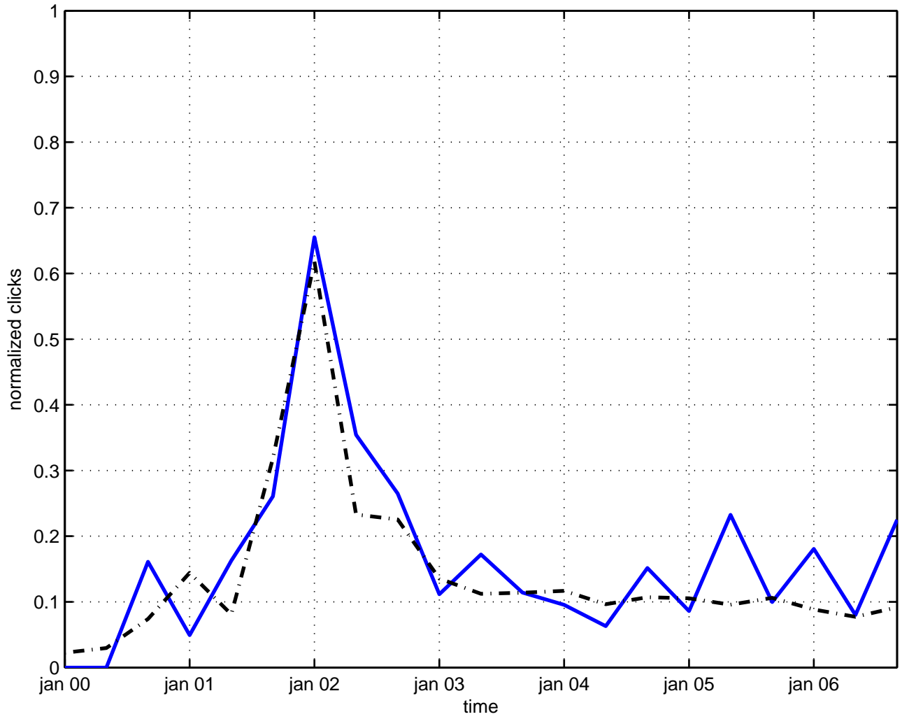
mass tachyon
