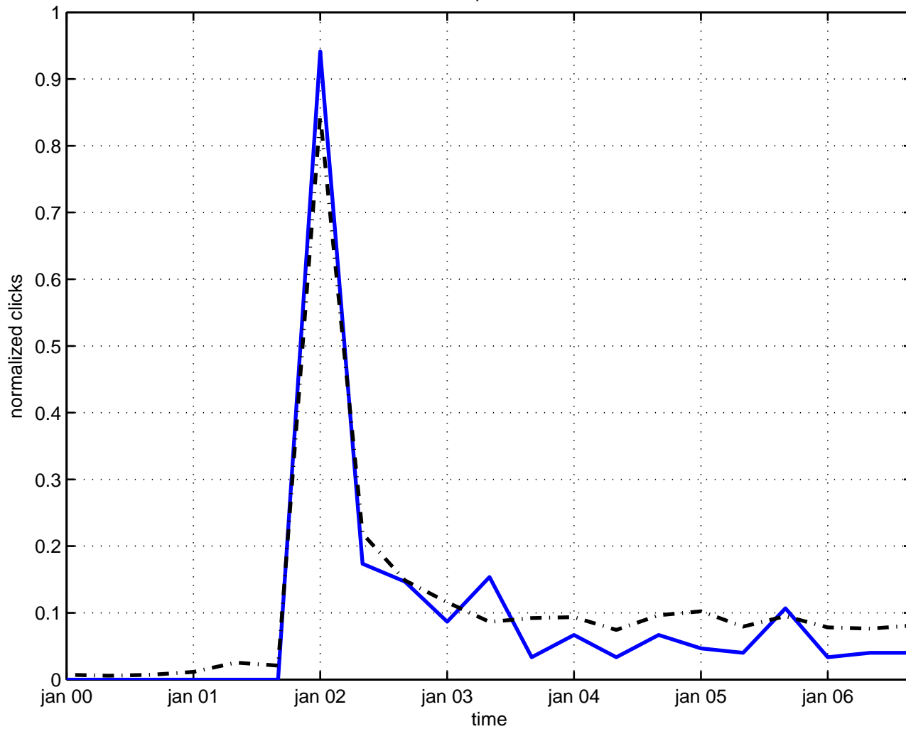
mass space-time
