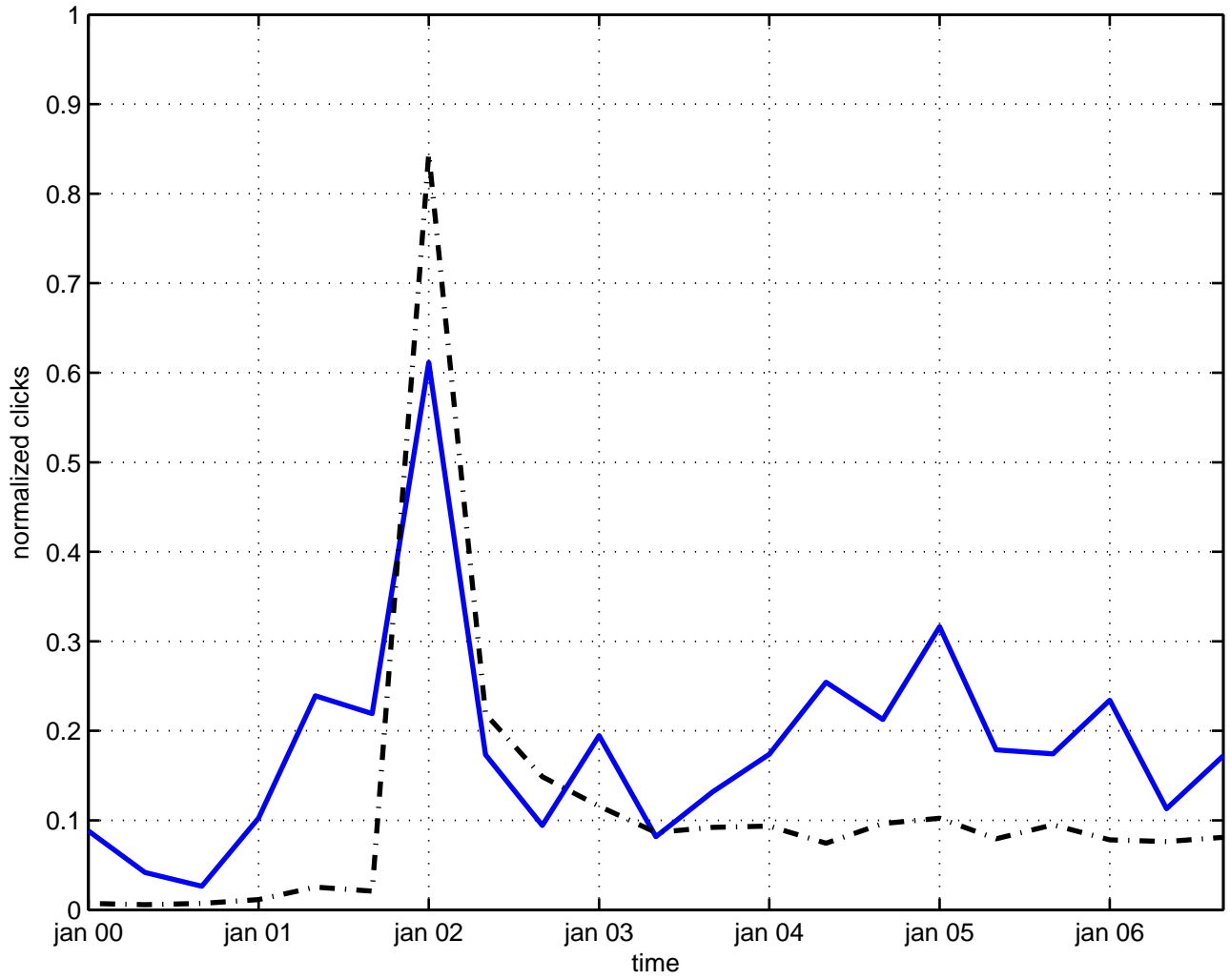
mass quark
