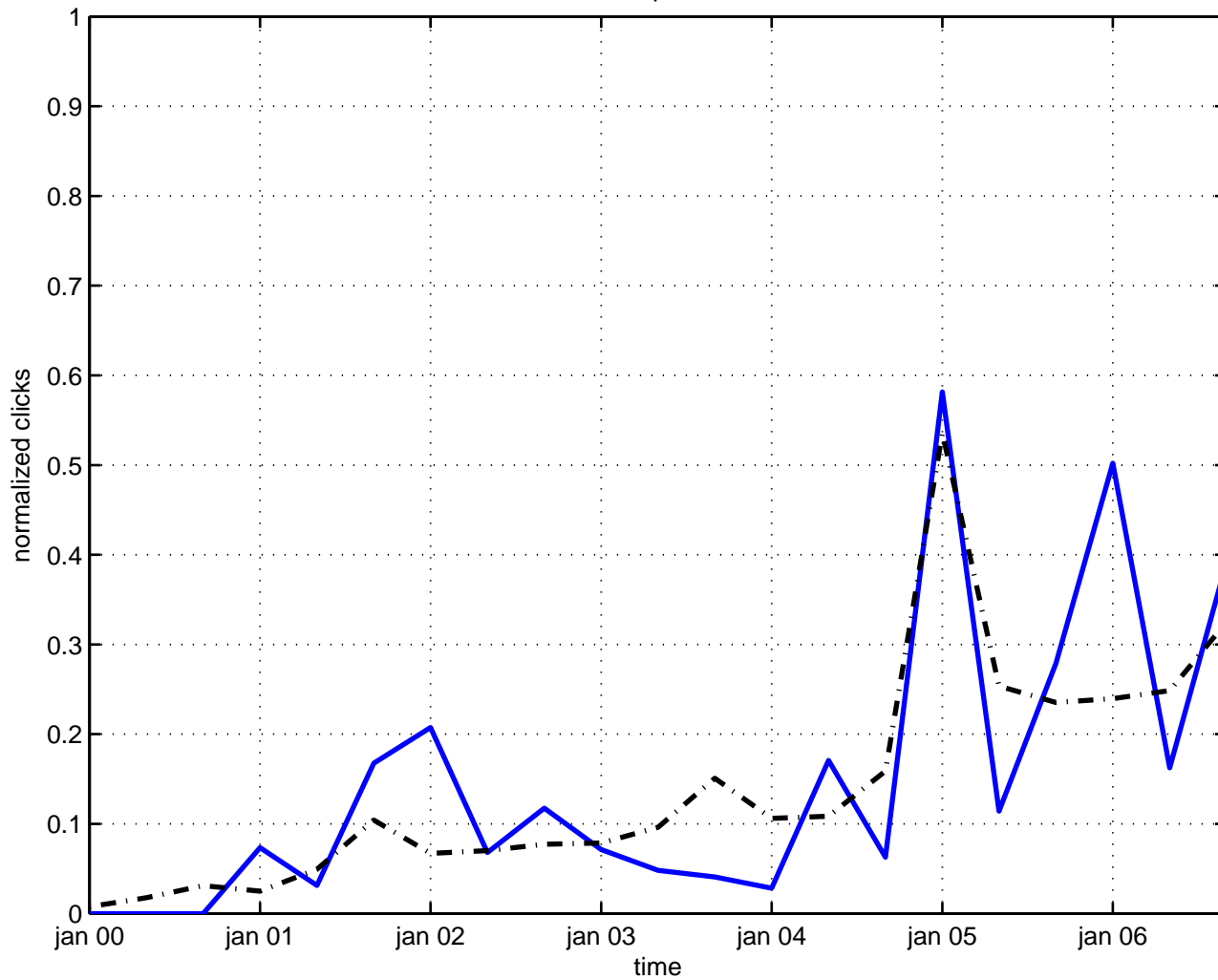
mass photon
